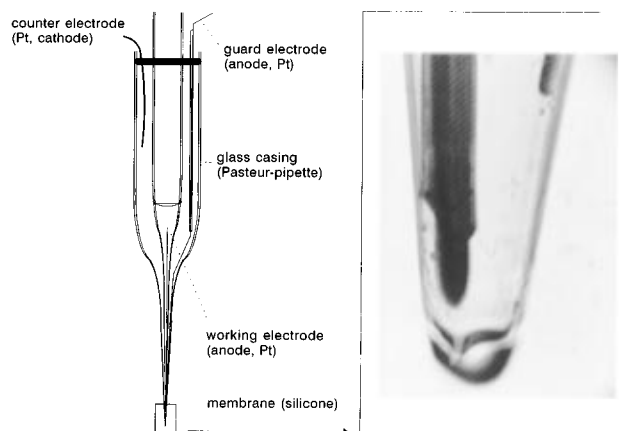
Figure 1. Amperometric microsensor.
