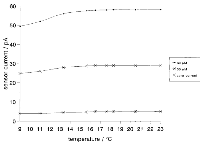
Figure 8. Influence of temperature on the sensor current.
