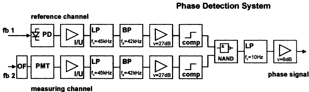
Fig. 1: Phase detection system (schematic drawing of analogue signal processing):
