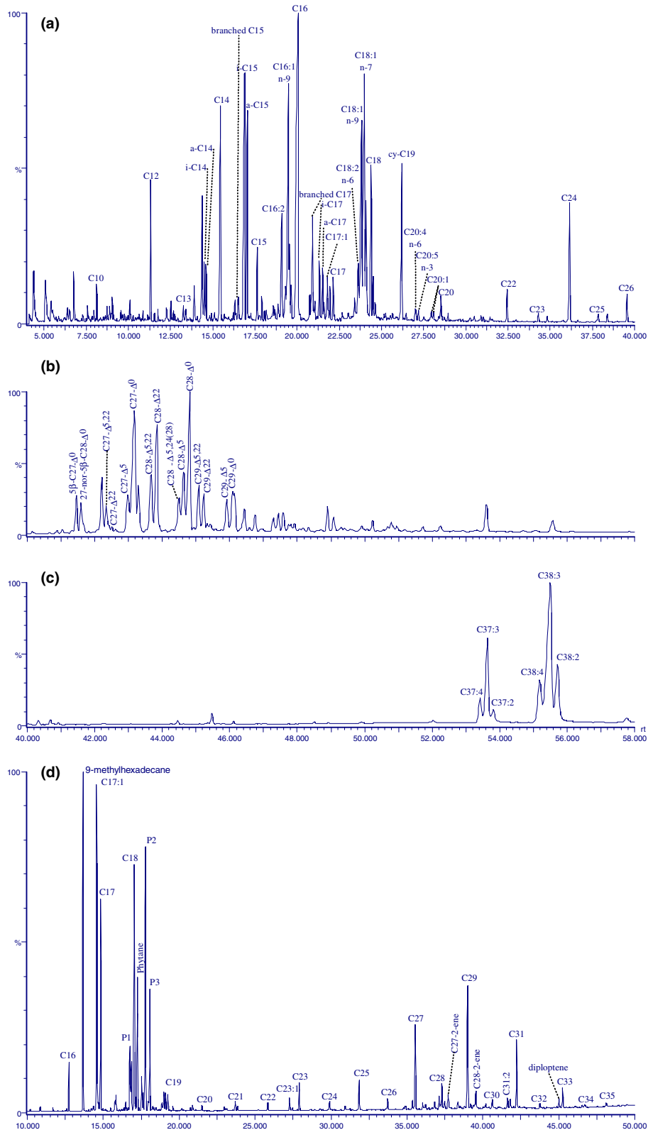
Fig. 3. Gas chromatographic profiles showing the major (a) fatty acids, (b) alcohol and (c) alkenone fractions, (d) hydrocarbons (P1, P2, P3 phytanes) from Salins-de-Giraud microbial mat.
